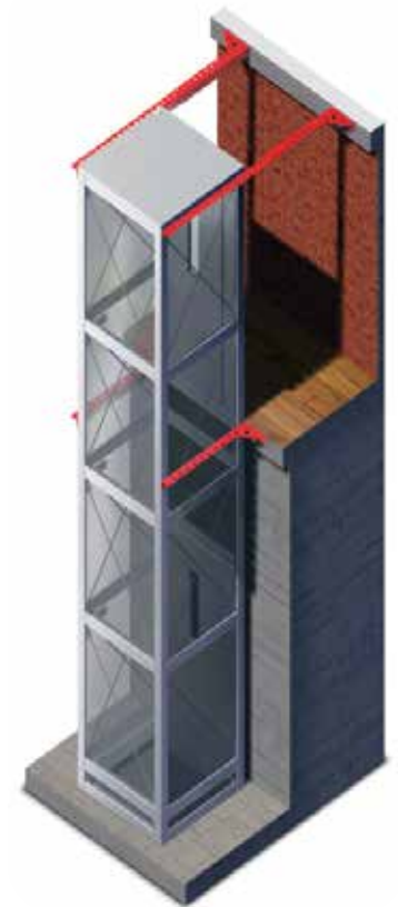
Brackets
